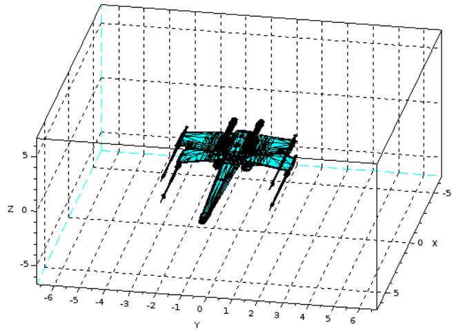
Xwing_fight.sce
